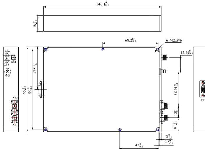
standard module package
